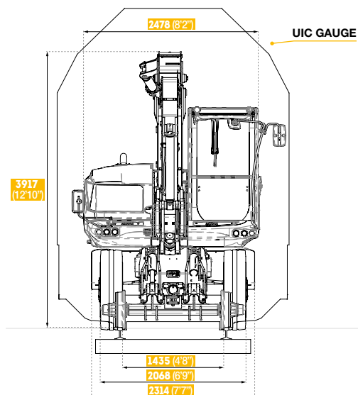
WORK POSITION - OVER THE FRONT, ALIGNED
