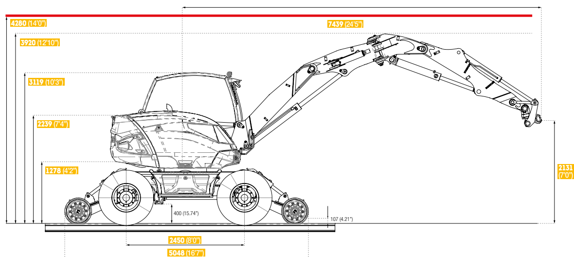
WORK POSITION - BELOW CATENARIES
